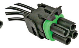
#5794PT (#5794C) Four Cavity Square Tower with Female Terminals
