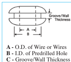
Flexible Oil Resistant Rubber Grommets Insert Into Predrilled Holes
