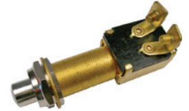
#5527PT (#5527C) Brass Marine Push-Button Momentary On SPST Starter & Horn Switch Chrome Plated Brass Button 2 Brass Screw Terminals 1-1/4" x 5/8" Mounting Stem 6 Volt 25 Amp 12 Volt 15 Amp
