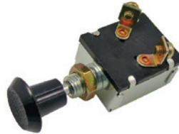
#5521PT (#5521C) On-Off Push-Pull SPST Short Style SPST 2 Screw Terminals 1/2" Mount Hole 6 Volt 25 Amp 12 Volt 15 Amp
