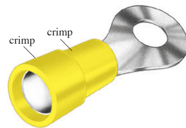
BUTTED SEAM BARREL NYLON INSULATION BRASS SUPPORT SLEEVE
